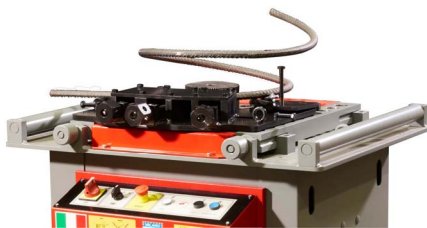
HEAVY DUTY SPIRAL DEVICE OPTIONAL Use with Up To #6 Bar
